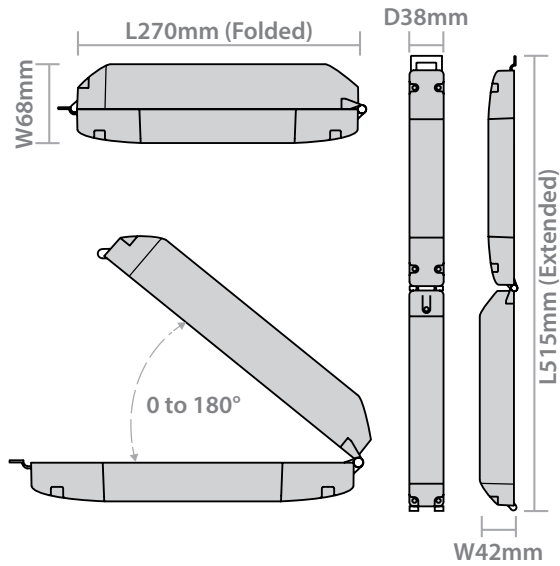
TITAN X/5/KIT/230 Dimensional Diagram
